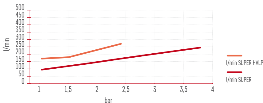
GRAFICO CONSUMO ARIA | AIR CONSUMPTION DIAGRAM GRAPHIQUE CONSOMMATION AIR | DIAGRAMM DES LUFTVERBRAUCHS
